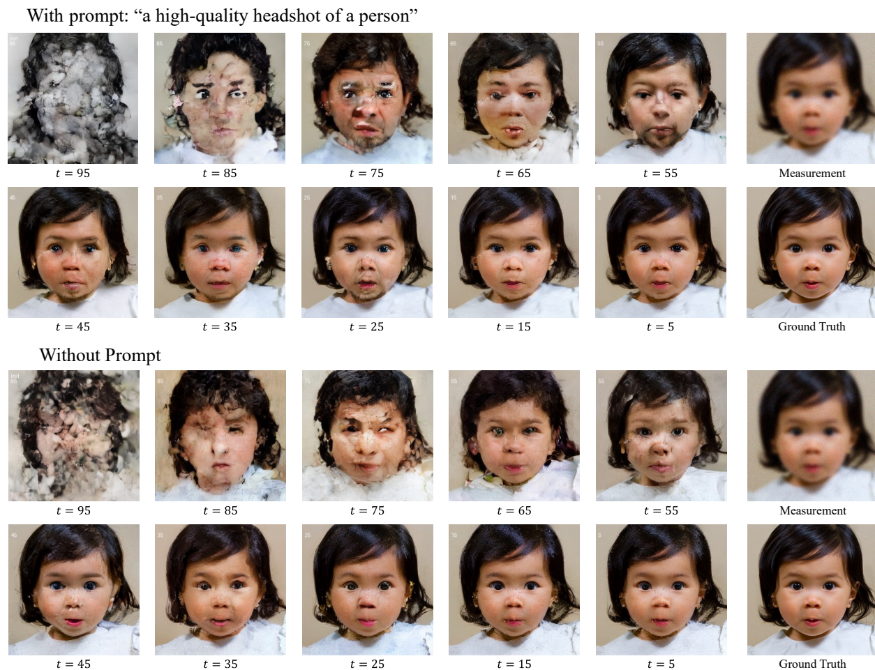
Figure 9: Failure modes of G2D2: Gaussian Deblurring results on the FFHQ dataset. Due to the mismatch between the prompt and the target image, errors remain uncorrected throughout the process, resulting in artifacts in the estimated image.
