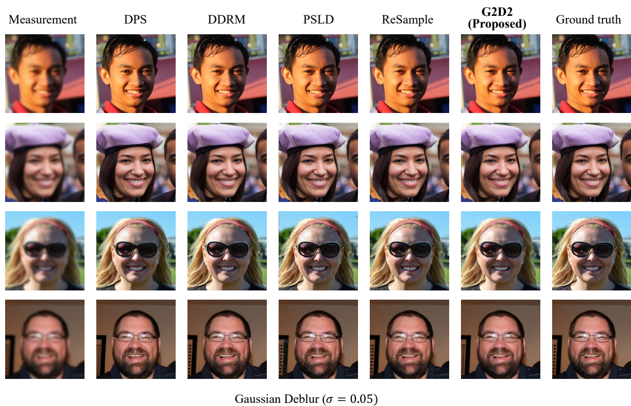
Figure 13: Qualitative results of G2D2 and comparison methods.
