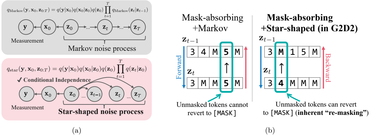
Figure 3: (a) Graphical model comparison between Markov noise process (top) and star-shaped noise process (bottom). The star-shaped model introduces conditional independence between z_t variables given z_0 , enabling more flexible error correction during sampling. (b) Comparison between mask-absorbing Markov process (left) and mask-absorbing star-shaped process (right). In the Markov process, unmasked tokens cannot revert to [MASK], while the star-shaped process allows tokens to naturally revert to [MASK] state (inherent “re-masking”), facilitating error correction in later sampling steps.
