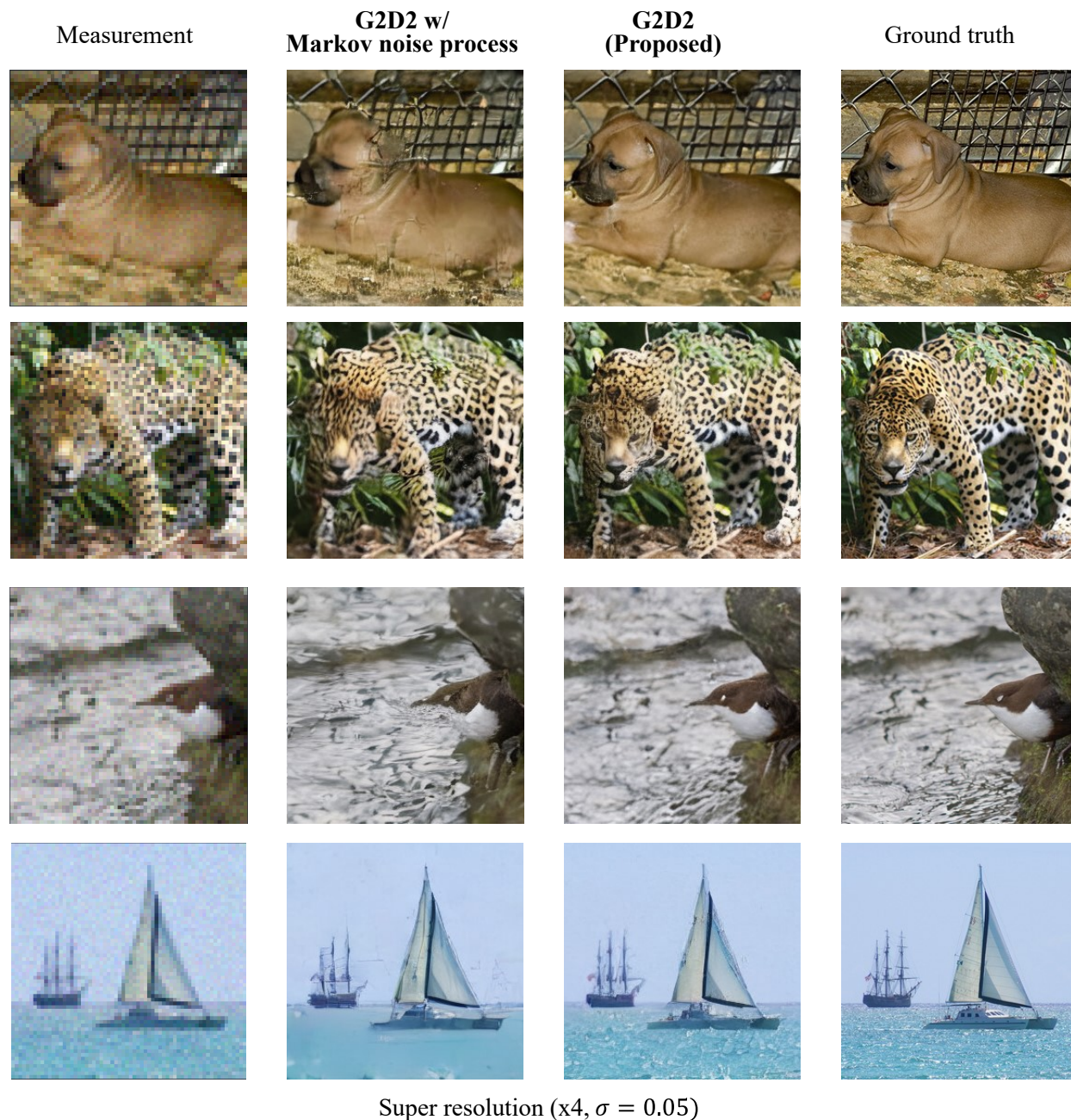
Figure 14: Qualitative results comparing G2D2 and G2D2 with Markov noise process (Super-resolution task).
