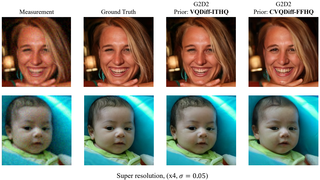
Figure 8: Qualitative comparison of super-resolution results ( \times 4 , \sigma = 0.05 ) on FFHQ test images. From left to right: low-resolution measurement, ground truth, G2D2 with VQDiff-ITHQ prior, and G2D2 with CVQDiff-FFHQ prior. While both prior models produce visually pleasing reconstructions, VQDiff-ITHQ prior tends to generate results closer to the ground truth, whereas CVQDiff-FFHQ prior produces fewer artifacts but with slightly less fidelity to the ground truth images.
