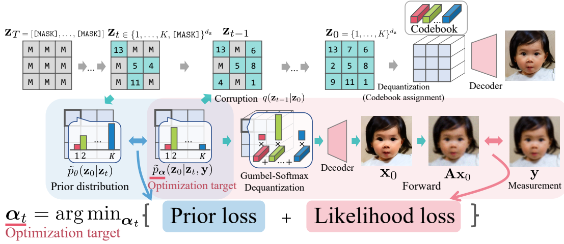
Figure 1: Illustration of G2D2. At each time step t , variational categorical distribution \tilde{p}_\alpha is optimized with respect to the sum of prior loss and likelihood loss, followed by sampling \mathbf{z}_{t-1} . Both terms are continuously differentiable, enabling continuous optimization.
