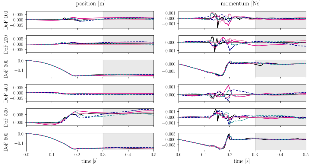
Figure 15. Predicted cloth positions and momenta for 6-dimensional RO-HNNs with latent dissipation matrix parametrized with a SPD network (—), a Cholesky network (---), and ground truth values (····), and 10-dimensional RO-HNNs with latent dissipation matrix parametrized with a SPD network (—), a Cholesky network (---), and ground truth values (····). The grey-shaded areas indicates interval beyond the data support.
