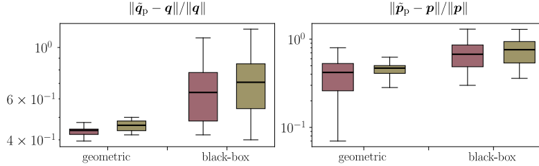
Figure 13. RO-HNN prediction errors ( \downarrow ) for black-box and geometric HNNs in latent spaces learned by a symplectic AE with latent dimensions d = 6 (■) and d = 10 (■) over 10 particle vortex trajectories.
