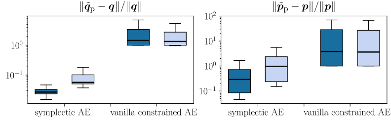
Figure 20. Prediction errors ( \downarrow ) of RO-HNNs with geometrically-constrained symplectic or vanilla constrained AE with Strang symplectic integrator (■) or Runge-Kutta integrator of order 4 (●) over 10 testing cloth trajectories.
