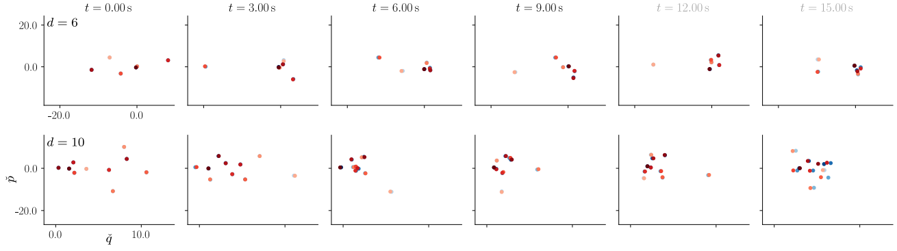
Figure 12. Predicted (•, •, •) vs ground truth (•, •, •) reduced positions of the particle vortex in the latent space of the RO-HNN with d = 6 and d = 10 . Times beyond 10s are out of the training data distribution.
