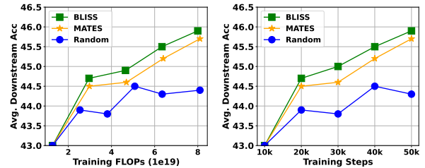
(a) Pretraining the 410M model.
