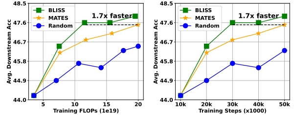
(b) Pretraining the 1B model.
