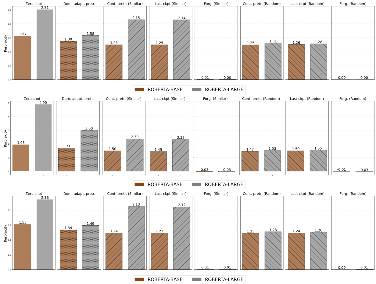
Figure 17: Above plots show the test perplexities (↓) with different RoBERTa sizes and training orders. For reference, we include the zero-shot and fine-tuning perplexities. The first panel shows the cumulative results, and the remaining two show the results obtained on Wiki and S2ORC domains. Inside the parentheses are the perplexity improvements over zero-shot (the smaller the better).
