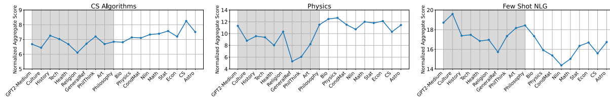
Figure 12: GPT2-M performance on the remaining three downstream tasks from BIG-Bench, captured at L1 domain transitions. The initial point represents the baseline performance of GPT2-M. The CS Algorithms and Physics results align with the findings in the main paper. For the Few-shot NLG task, performance trends across Wiki and S2ORC domains do not follow a consistent pattern. A deeper inspection reveals that domains such as Culture, Art, Philosophy, Math, Stat, and Econ contribute positively to performance enhancement in this task.
