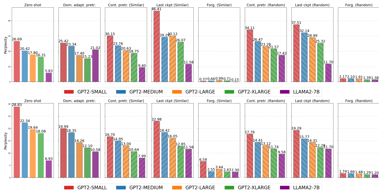
Figure 16: A more detailed analysis of our main results table. This time, we compute the test perplexities(↓) on Wiki and S2ORC portions separately, visualized in the upper and lower panels.
