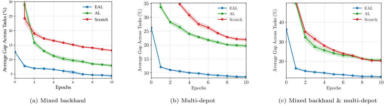
Figure 7: Validation gaps averaged across new tasks including unseen features (a) mixed backhaul (MB), (b) multi-depot (MD), and (c) their combination (MB&MD) for retraining from scratch, AL and EAL finetuning.
