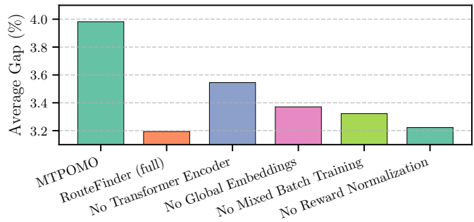
Figure 5: Ablation study on ROUTEFINDER components.
