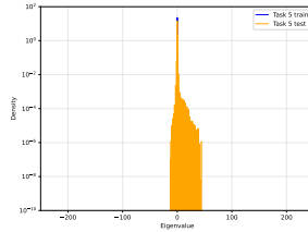
(k) L2: task 5
