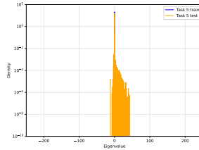
(h) CBP: task 5
