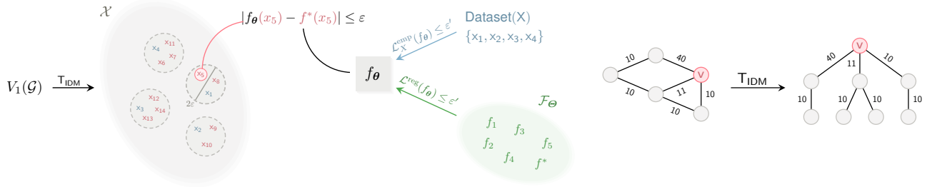
Figure 1. An illustration of the learnability result in Theorem 2, applied to MPNNs by first mapping the space V_1(\mathcal{G}) to a pseudometric space (via IDMs or computation trees; see Section K.1), satisfying Definition 1 and then applying Theorem 2. A computation-tree construction is shown on the right.
